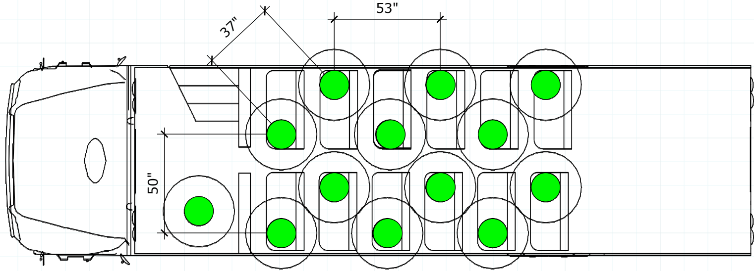
SPECIAL ED BUS 13 BODIES (INCLUDING DRIVER)
